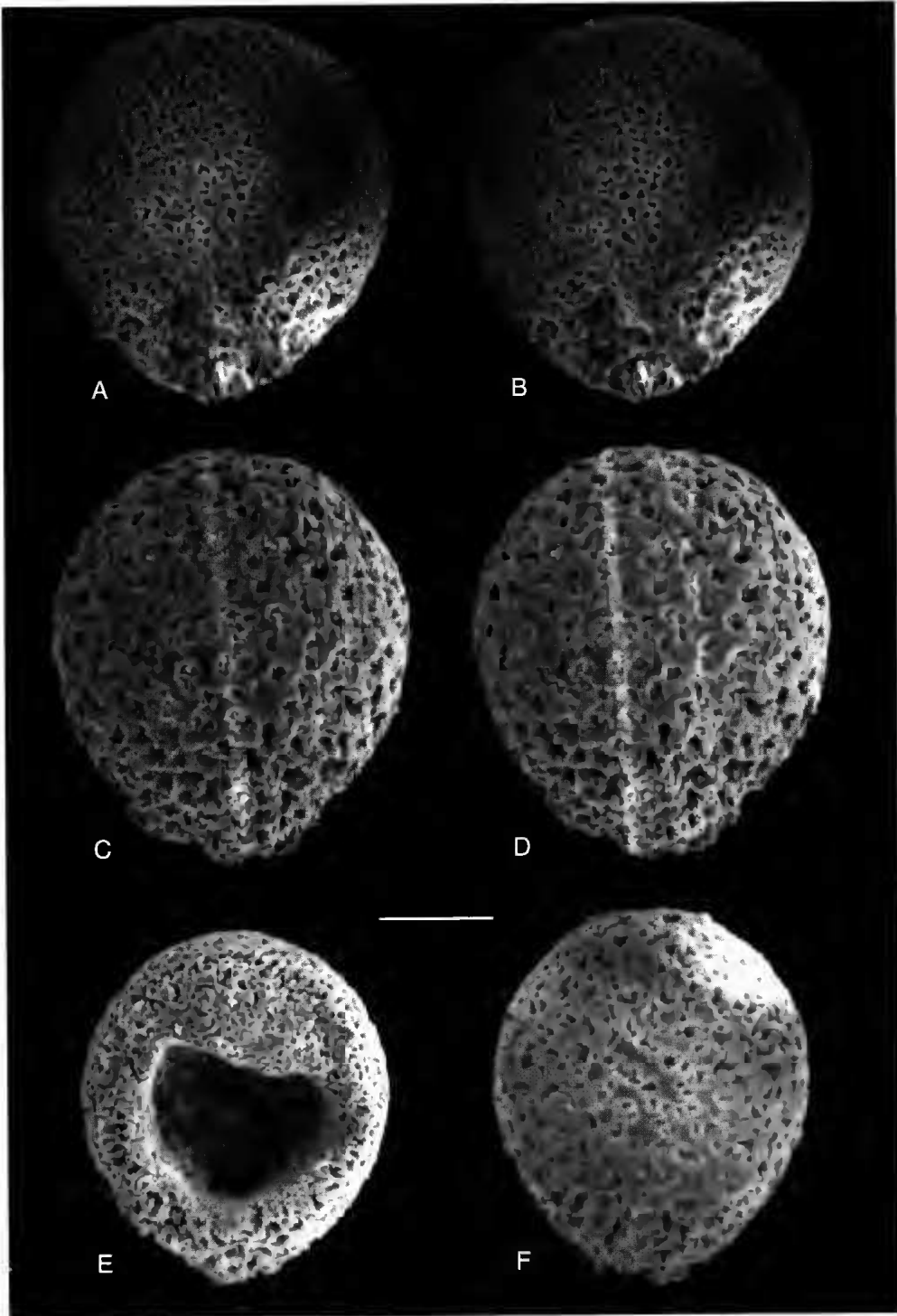
FIG. 10. — Glomeropyle poinui Aita, n. sp.; A, B, holotype, stereograph (photo Nos 31104, 31105); C, D, paratype stereograph (photo Nos 31126, 31127); E, paratype (photo No. 31128); F, photo No. 31135. Sample MAH-3.5, Unit 2, Mahinepua Peninsula, North Island, New Zealand. Scale bar: 100 \mu m.
